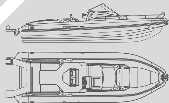
Design by: Cantieri Capelli's technical dept.
